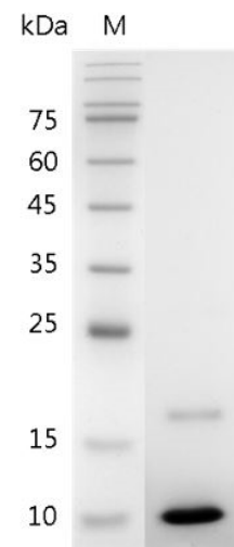
SDS-PAGE analysis of recombinant mouse IGF-I
